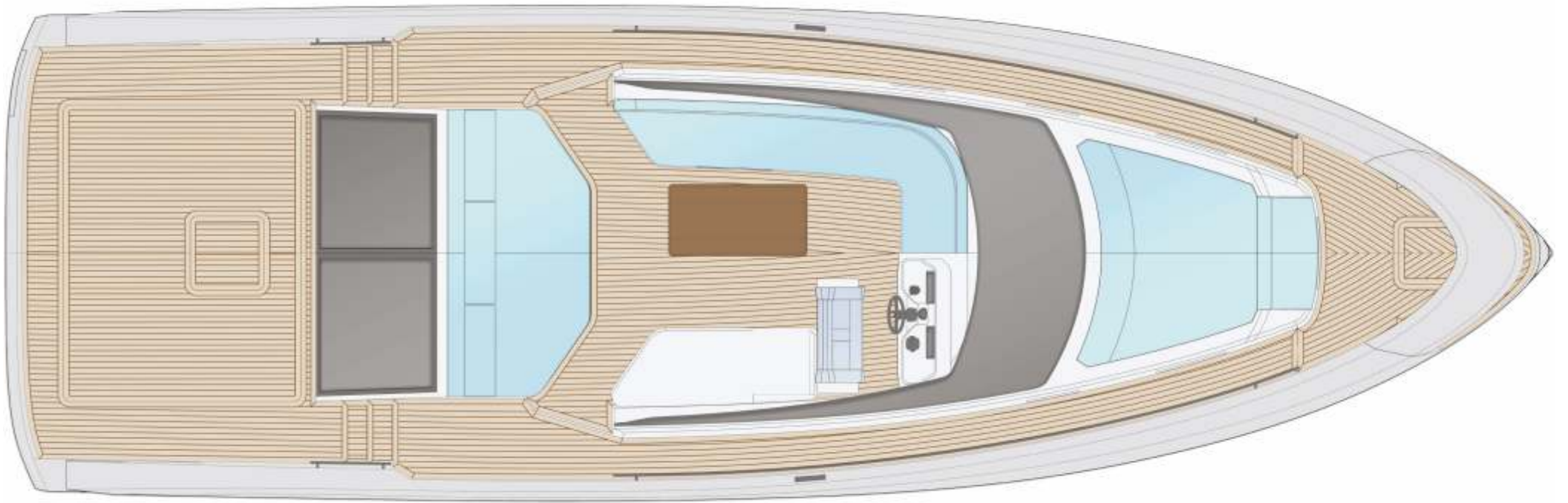
MAIN DECK
