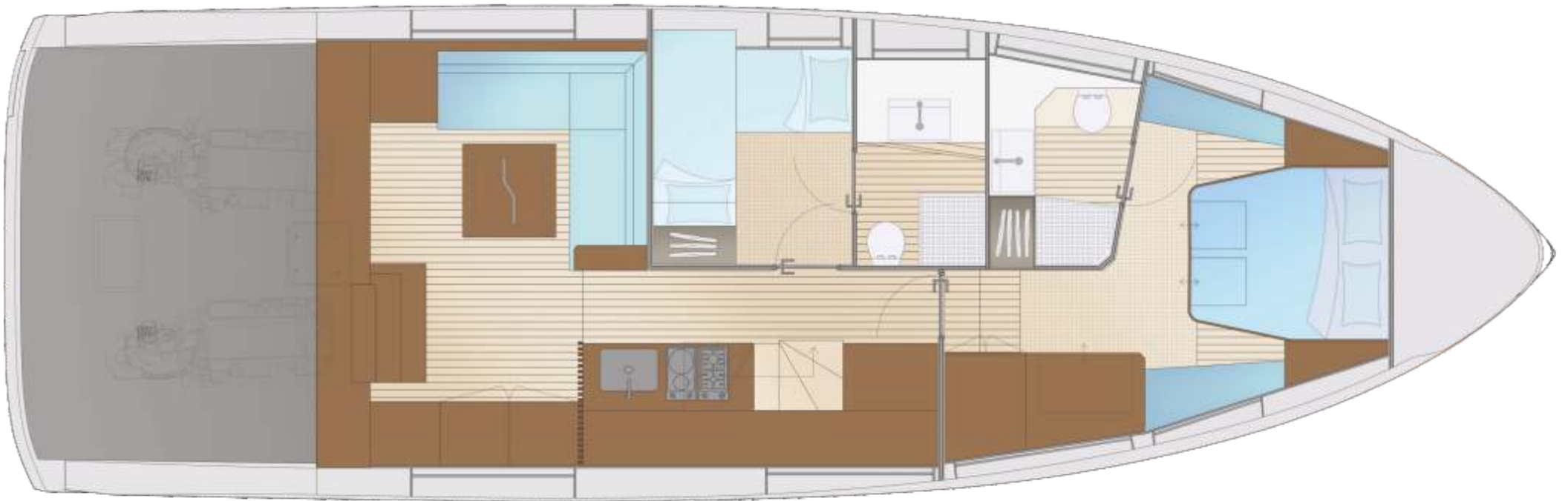
LOWER DECK
