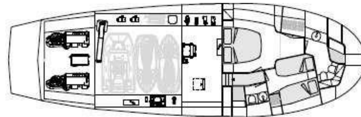
LOWER DECK 2 Cabins version Versione 2 cabine
